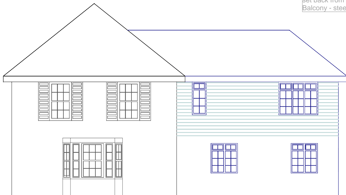
PROPOSED EAST ELEVATION (FRONT)
